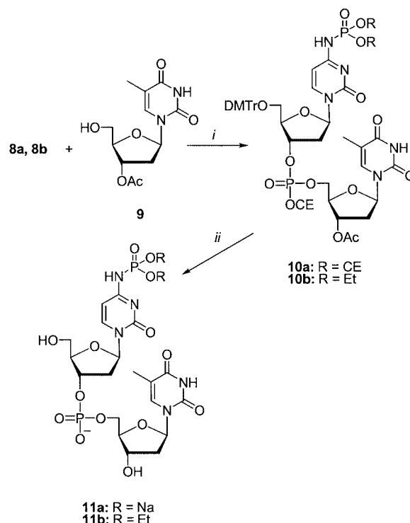
Scheme 2. (i) (a) 1 H -tetrazole, CH 3 CN, room temp., 30 min; (b) t BuOOH, CH 3 CN, room temp., 15 min. (ii) (a) concd. NH 3 /pyridine (3:1), room temp., 12 h, (b) 80% AcOH, room temp., 30 min; CE = 2-cyanoethyl
