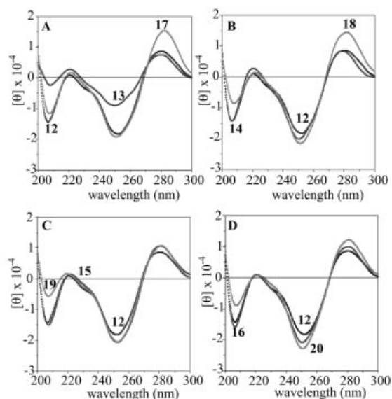
Figure 3. The CD spectra of oligodeoxynucleotides containing N -phosphorylated deoxycytidine derivatives: A : d(CGCGAATTCGCG); B : d(CGCGAATTCGCG); C : d(CGCGAATTCGCG) D : d(CGCGAATTCGCG)
