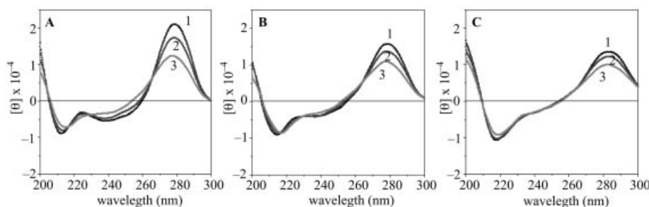
Figure 2. CD spectra of d(C*pT) dimers observed at various temperatures: 1: 0 °C; 2: 20 °C; 3: 60 °C; A: d(CpT); B: d(C*pT) ( 11a ); C: d(C**pT) ( 11b )
