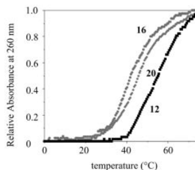
Figure 4. Melting temperatures of oligodeoxynucleotides containing N -phosphorylated deoxycytidine derivatives
