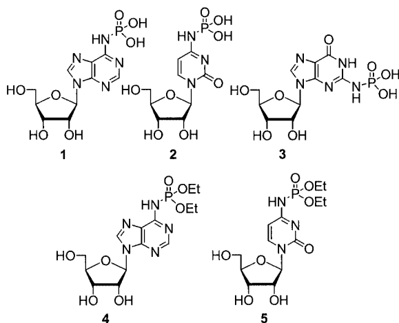
Figure 1. N -Phosphorylated ribonucleoside derivatives
